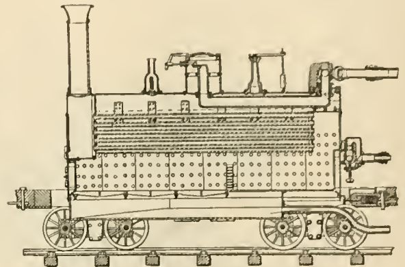
BOILER OF NICHOLS' NOVELTY FIG. 71.
